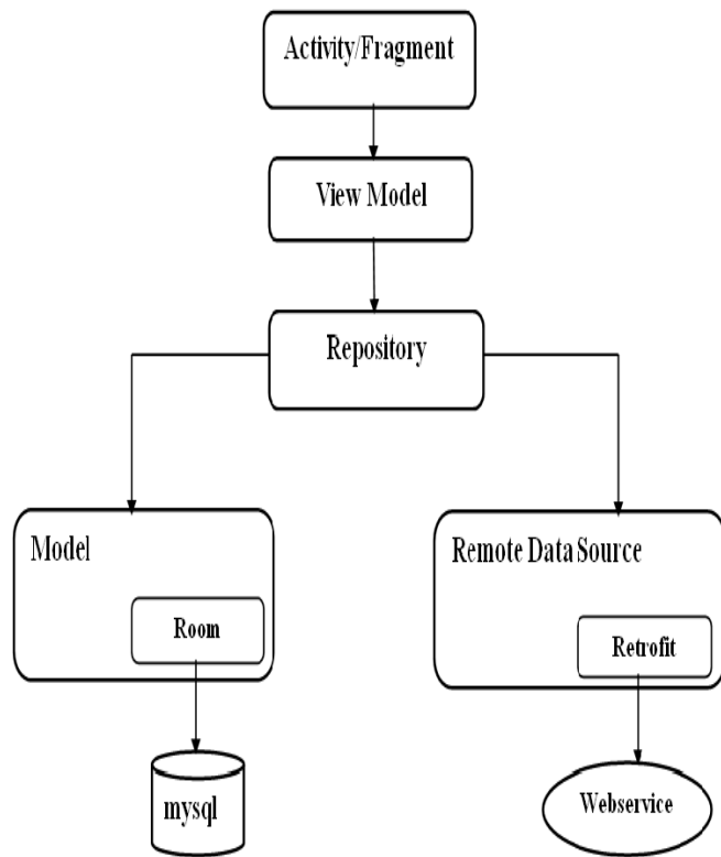
Figure 1: Architecture Diagram
